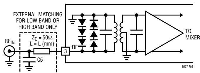
Figure 3. RF Input Schematic
