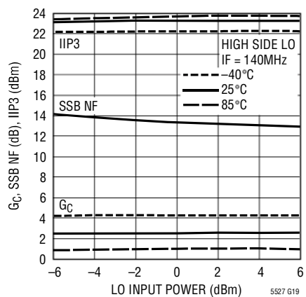
450MHz Conversion Gain, IIP3 and NF vs LO Power
