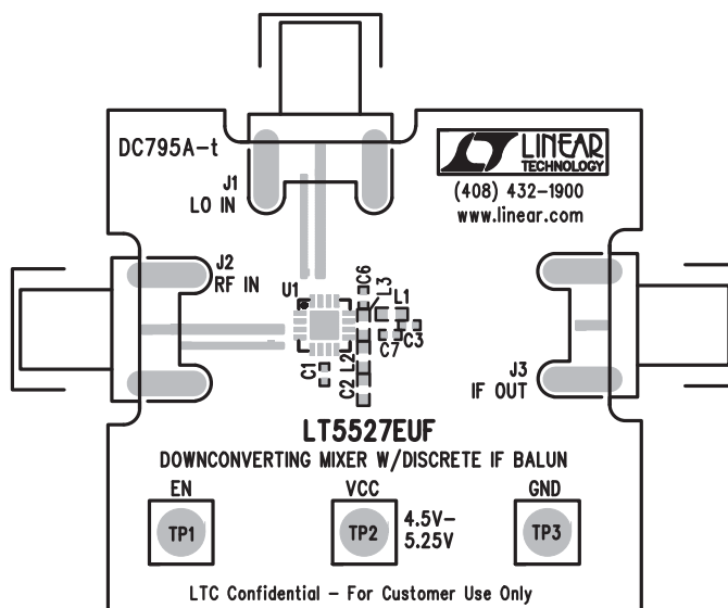
Discrete IF Evaluation Board Layout
